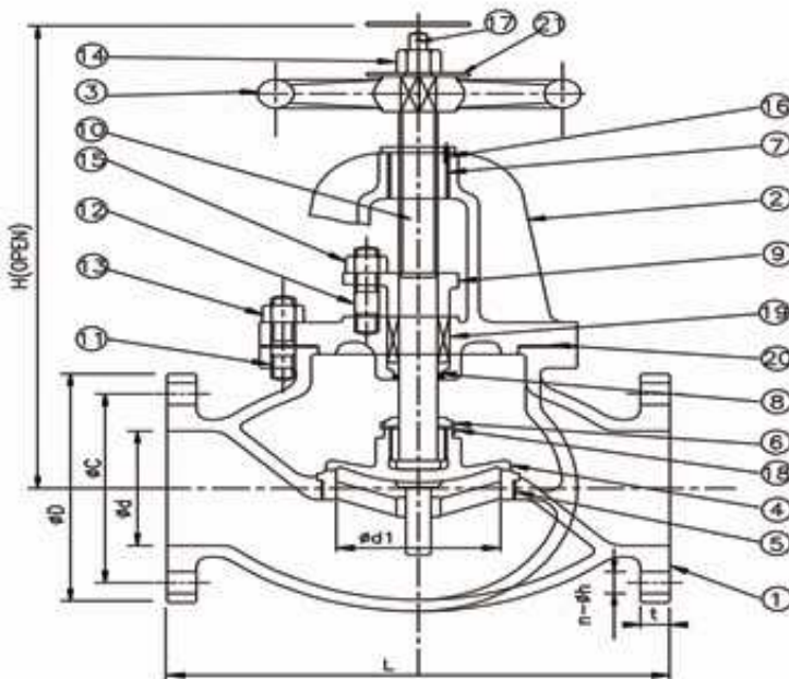
DIMENSION (5K:F7305, 10K:F7307)
